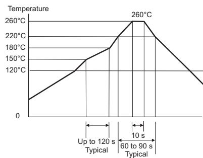
Figure 7 Solder Profile
